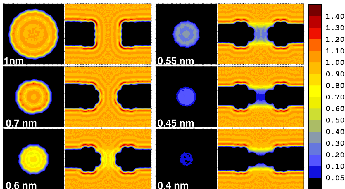
Figure 3.6: Water density in hydrophobic pores with radii ranging from 1.0 nm to 0.4 nm. Left column in each panel: density z-averaged over the length of the pore. Right column: radially averaged density. The density is in units of SPC bulk water at 300 K and 1 bar. Note that for the R = 1.0 nm, 0.7 nm, and 0.4 nm pore the membrane mimetic slab had a thickness of four methane layers but for technical reasons only three layers were used in the other cases. (Plots were prepared with xfarbe 2.5 (Ref. 223))
